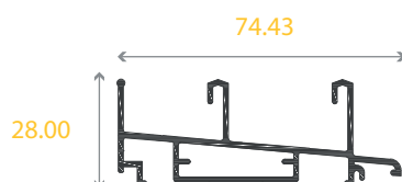
3640 Marco
